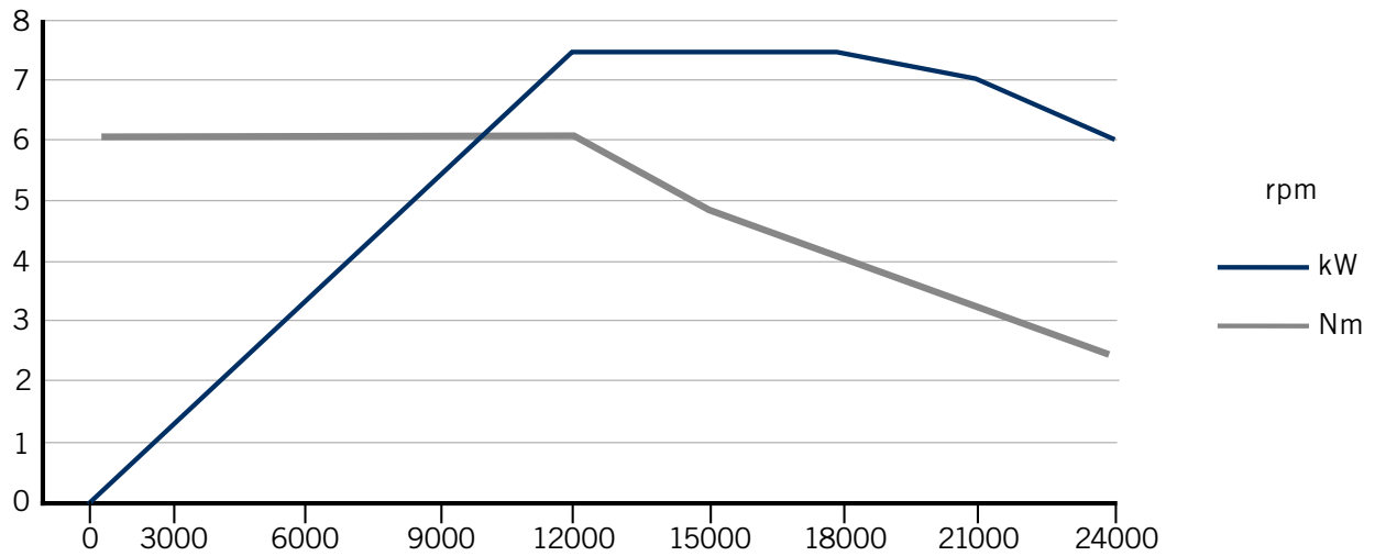
Power - Torque S6
